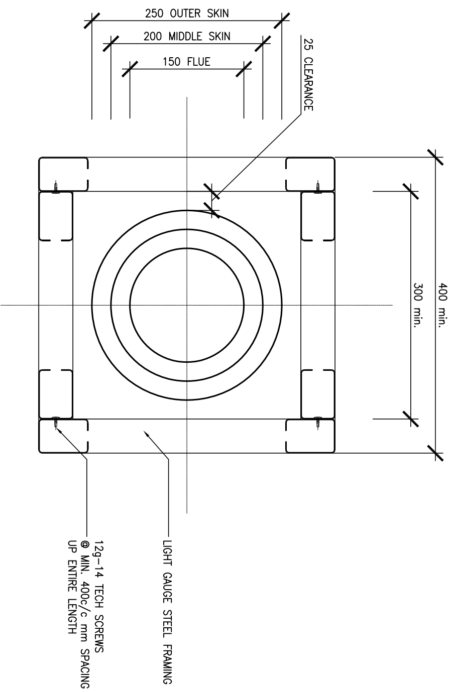
PLAN VIEW OF CHIMNEY FRAME ASSEMBLY
